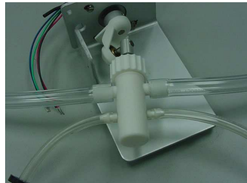
Example of pump with rinse ports at rear of pump (note: hose clamps have been removed for photo clarity).
